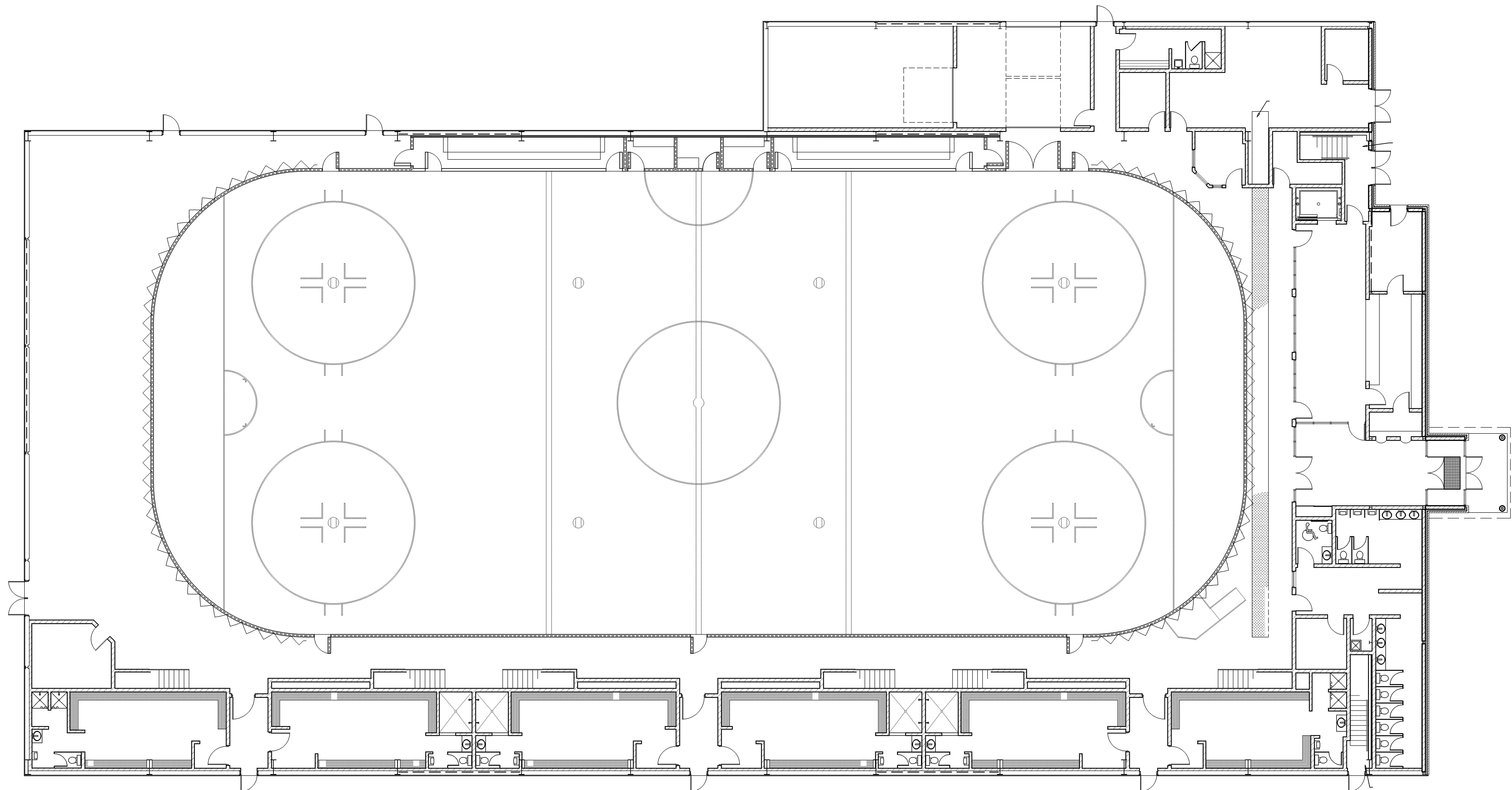
MAIN FLOOR PLAN SCALE: 1/8" = 1'-0"
